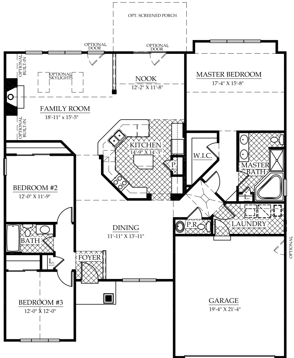
FIRST FLOOR PLAN 2040 SQ. FT.
